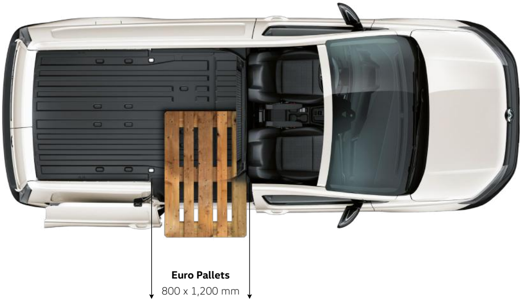
Wider Maxi sliding door (846 x 1,095 mm) for Caddy Cargo Maxi¹
