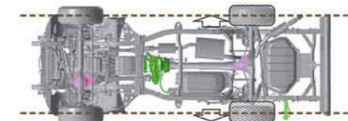
front tread (1605mm)
